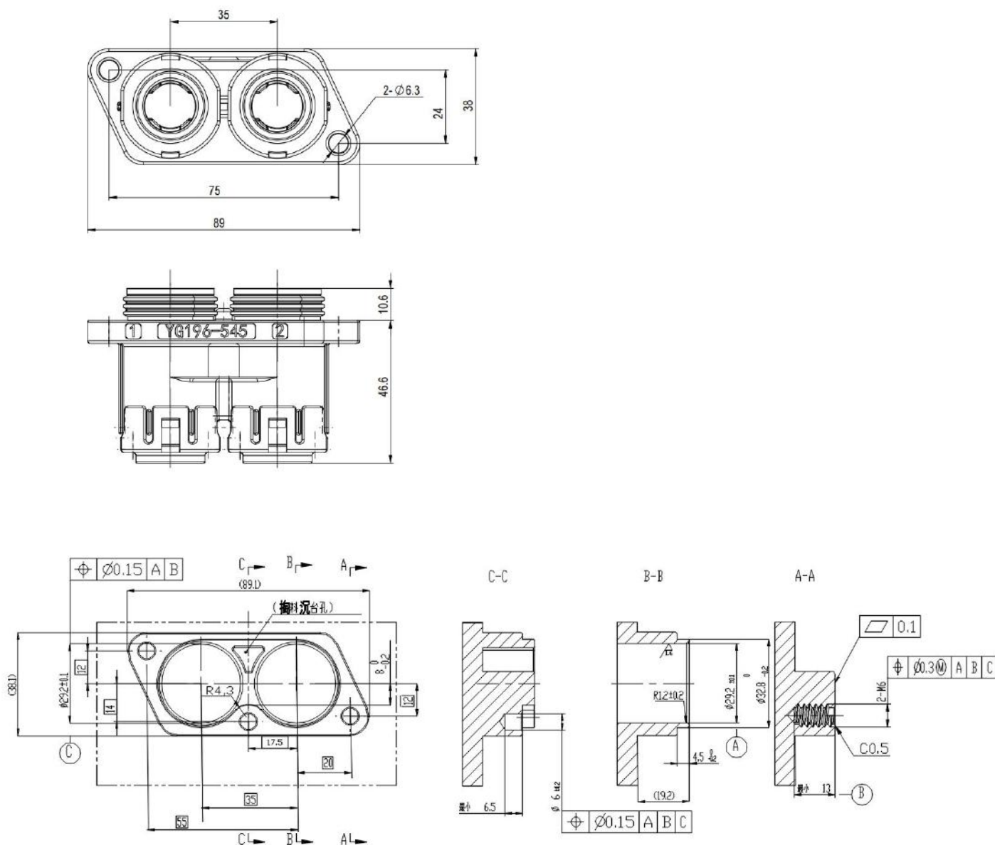
面板开孔尺寸 Panel mounting hole dimension
