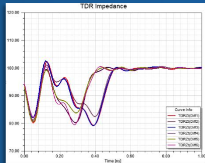
Signal Integrity
