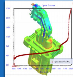
Mold flow
