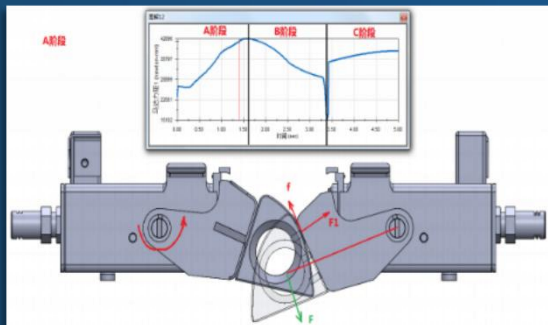
Structure strength
