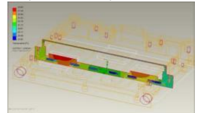
Liquid Cooling Module Cross-Sectional Temperature Heat Map
