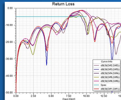
Signal Integrity
