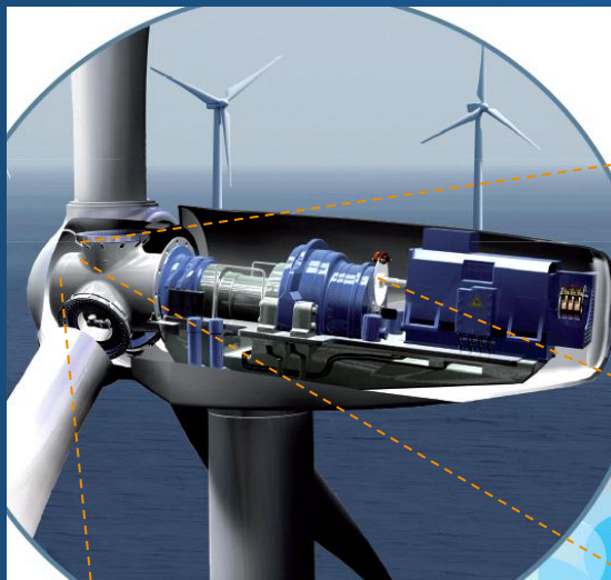
Pitch system
